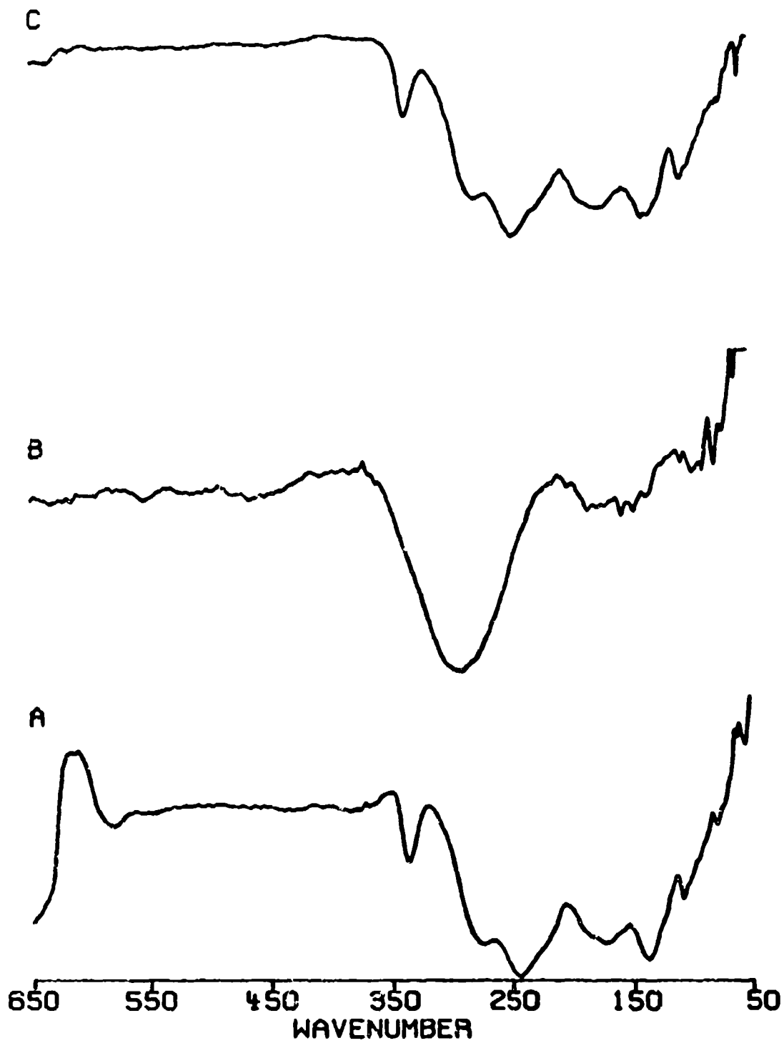
Figure 43. Far IR of Sb_2S_5 (A) Sb_2S_3 ; (B) Sb_2S_5 ; (C) Sb_2S_5 at 270^\circ C in N_2 .
