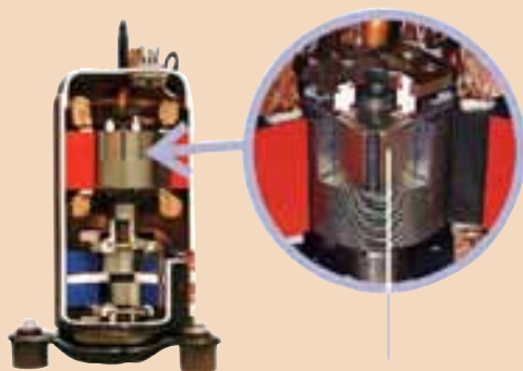
Neodymium magnets
