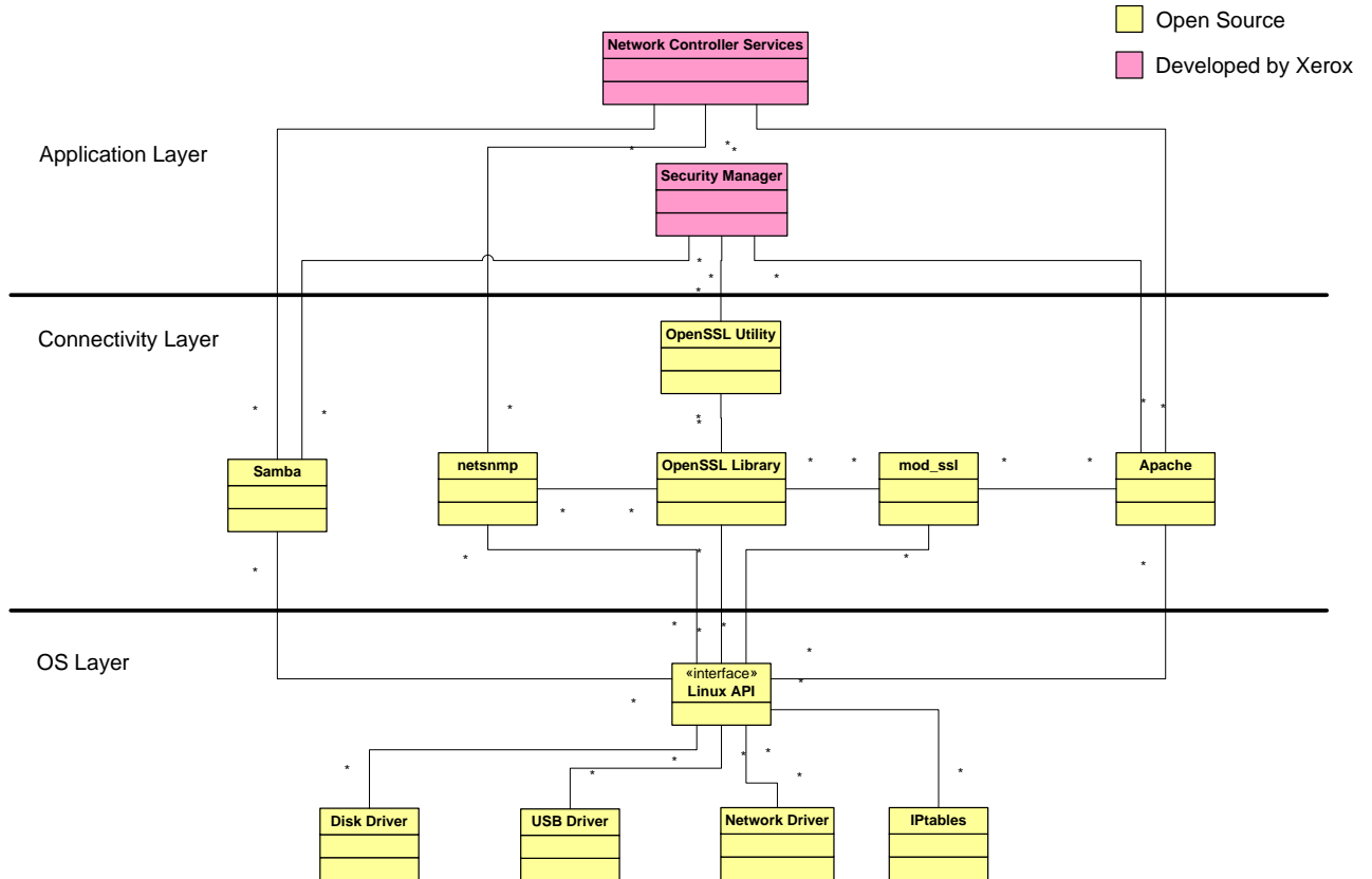
Figure 2-3 Controller Operating System layer components
