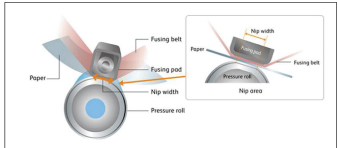
Fuser Belt Pressure and Heat Control
