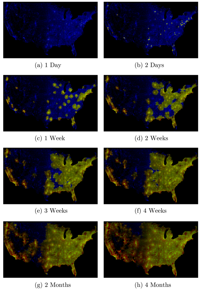
FIG. 11. (Color online) Simulation of a zombie outbreak in the continental United States. Initially one in every million individuals was infected at random. Results are shown above at (a) one day, (b) two days, (c) one week, (d) two weeks, (e) three weeks, (f) four weeks, and (g) two months after the outbreak begins. Shown here are the population of susceptible individuals ( S ) in blue, scaled logarithmically, zombies in red, and removed in green. All three channels are superimposed. A movie version of this outbreak is available in the Supplemental Materials online [26].
