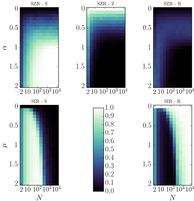
FIG. 5. (Color online) Mean final states as a function of model parameters. One thousand different simulations are run for each cell. Each simulation starts with a single zombie or infected individual. The runs are run until they naturally terminate, either because the susceptible population is deleted, the zombie population is gone, or there are no more infected individuals. Each cell is colored according to the mean fraction of the population occurring in each state. The top row is for SZR simulations and the bottom row is for SIR simulations. In both cases N is chosen to be 100. Here the sharp contrast between density-dependent SZR and SIR is made apparent. Notice that density-dependent SIR is very strongly population dependent.
