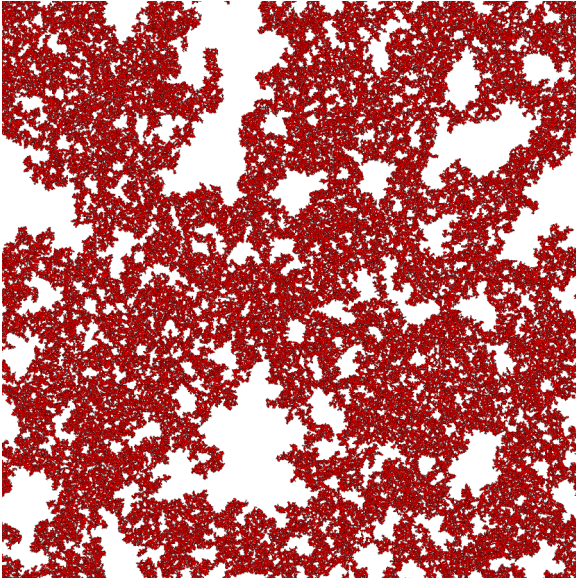
FIG. 6. (Color online) Example cluster resulting from the single population per site square lattice zombie model with periodic boundary conditions near the critical point \alpha_c = 0.43734613(57) on a lattice of size 2048 \times 2048 . Susceptible, infected (zombie), and removed are shown in white, red, and black, respectively.
