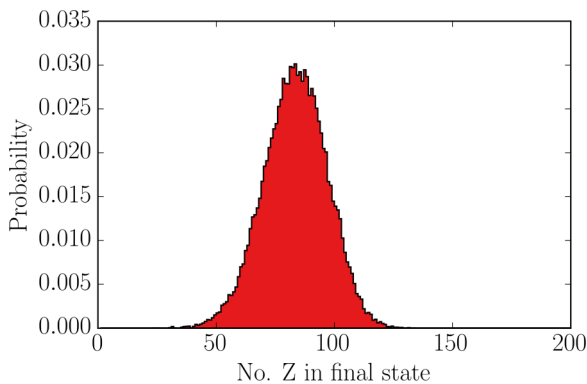
FIG. 3. (Color online) Distribution for final zombies over 100 000 stochastic trajectories with the same parameters as Fig. 2. Not pictured are the 60% of runs that end with no zombies in the final state. Compare these to the analytical result, in which the final population of zombies would be 81 with no possibility of surviving humans.
