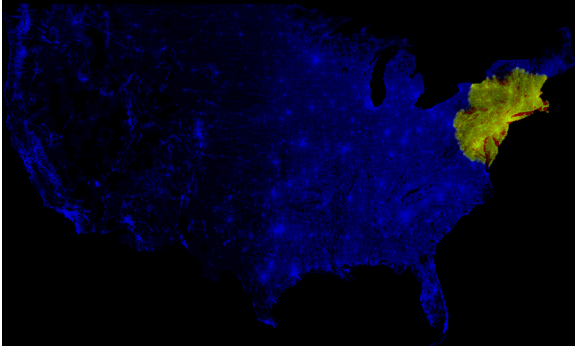
FIG. 12. (Color online) Status of the United States 28 days after an outbreak that started in New York City. Here blue represents humans, red represents zombies, and green represents dead zombies. The three color channels have been laid on top of one another.
