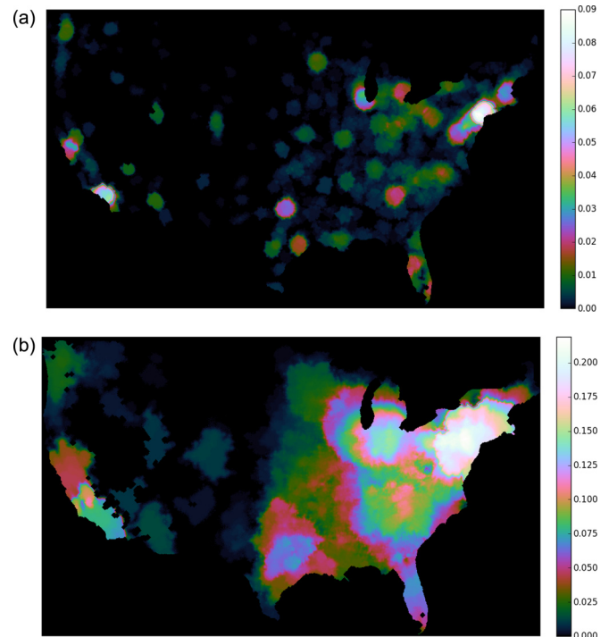
FIG. 13. (Color online) Average infection rate from US scale runs. In both cases, the plot shows the probability of being infected in that square after an epidemic that originates from a single infected individual chosen at random from the total population. The top figure (a) is the probability of being infected after 7 days, while the bottom plot (b) is after 28 days. In total, this represents 7000 simulated runs starting from a single individual. The top plot represents the 1467 outbreaks that lasted at least 7 days; the bottom plot represents 1458 outbreaks that lasted at least 28 days.
