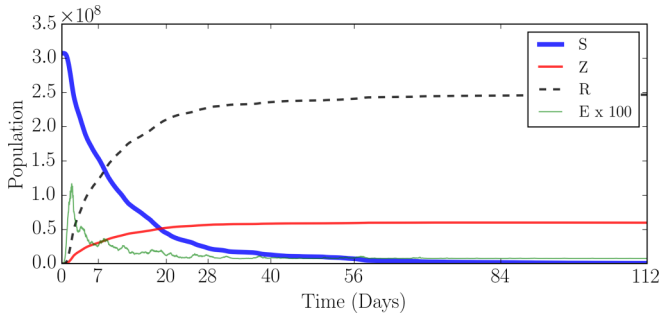
FIG. 10. (Color online) S (thick solid blue), Z (solid red), R (dashed black), and E (light thin green) populations as a function of time for a full scale zombie outbreak in the continental United States starting with one in every million people infected. The exposed population ( E ) has been magnified by a factor of 100.
