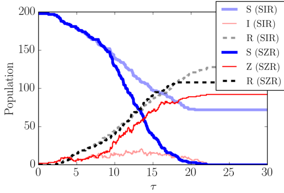
FIG. 2. (Color online) Example Gillespie dynamics for the SIR and SZR models with the same parameter settings as Fig. 1. The (susceptible, infected, removed) population is shown in (thick blue, thin red, dashed black). The SZR results are dark lines, while the SIR results are lighter lines. The two simulations were run with the same seed so as to match their dynamics at early times.
