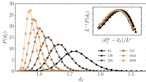
FIG. 8. (Color online) Histograms of P(d_f|L) , the observed fractal dimensions of the zombie epidemic clusters as measured by box counting, measured in L \times L systems sizes L varying from 64 to 2048. These extrapolate to give a measured value consistent with the exact percolation value 91/48 , with an error of \pm 0.04 . The inset shows a finite-size scaling collapse of these same curves. Using scale invariance arguments similar to those in the text, one can argue that properties like our measured d_f should take the form P(d_f|L) \sim L^x \mathcal{P}((d_f^{\infty} - d_f)/L^x) . Hence by multiplying P(d_f|L) by L^{-x} and plotting it versus (d_f^{\infty} - d_f)/L^x , the scaling theory predicts the curves at large system sizes should all lie atop one another. Here we estimate the critical exponent x \sim 0.30 \pm 0.05 ; we also used the scaling collapse to extrapolate and measure d_f .
