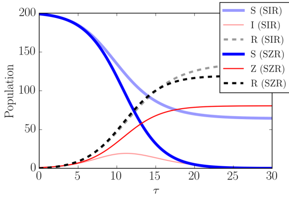
FIG. 1. (Color online) Deterministic trajectories for the SIR and SZR models with an initial population of 200 people, 199 uninfected and 1 infected. The (susceptible, infected, removed) population is shown in (thick blue, thin red, dashed black). The SZR results are darker lines, while the SIR results are lighter lines. For both models \tau = t\beta N , where N was taken to be the total population. For the SZR model \alpha was chosen to be 0.6, while for the SIR model \mu was chosen to be 0.6 to show similar dynamics. Notice that, in this case, in SZR the human population disappears and only zombies remain in the end, while the SIR model is self-limiting, and only a fraction of the population ever becomes infected.
