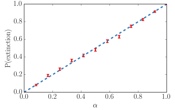
FIG. 4. (Color online) Observed fraction of simulations that end in an extinction for the zombie outbreak, for 1000 runs of 10^4 individuals at various values of \alpha [Eq. (33)]. The observed extinction probabilities agree with the expectation that they should go as \alpha , here shown as the dashed line. This is the same behavior as the SIR model.
