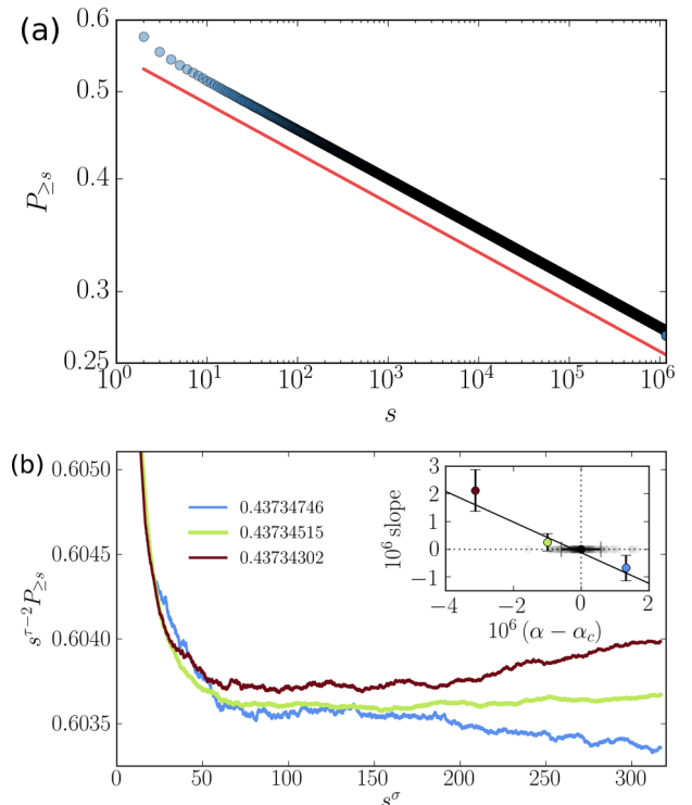
FIG. 7. (Color online) Cumulative distribution of epidemic sizes for the two dimensional zombie model near the critical virulence. The critical point found was \alpha_c = 0.43734613(57) . (a) The probability of a site being in a cluster of at least s in size ( P_{\geq s} ) is shown in blue circles. The fact that it forms a straight line on a log-log plot indicates that P_{\geq s} is a power law, and the slope is 2 - \tau . For comparison, the red line shows the power law corresponding to the percolation critical exponent: \tau = 187/91 . (b) Data for three different values of \alpha near \alpha_c , each times s^{\tau-2} using the exponent from percolation theory that should make the critical point into a flat line. We plot these against s^{\sigma} , the size taken to the power law \sigma = 36/91 , as in Ref. [20]. Notice that for \alpha > \alpha_c (when the zombies lose) the large outbreaks are suppressed below the power law, and for \alpha < \alpha_c (when the zombies often win) the largest outbreaks bend up. We follow Ref. [20] in estimating \alpha_c by interpolating these slopes; the inset shows a bootstrap estimate of our error in \alpha_c . Notice that the three curves are for very similar \alpha —leading to excellent precision in identifying the critical point.
