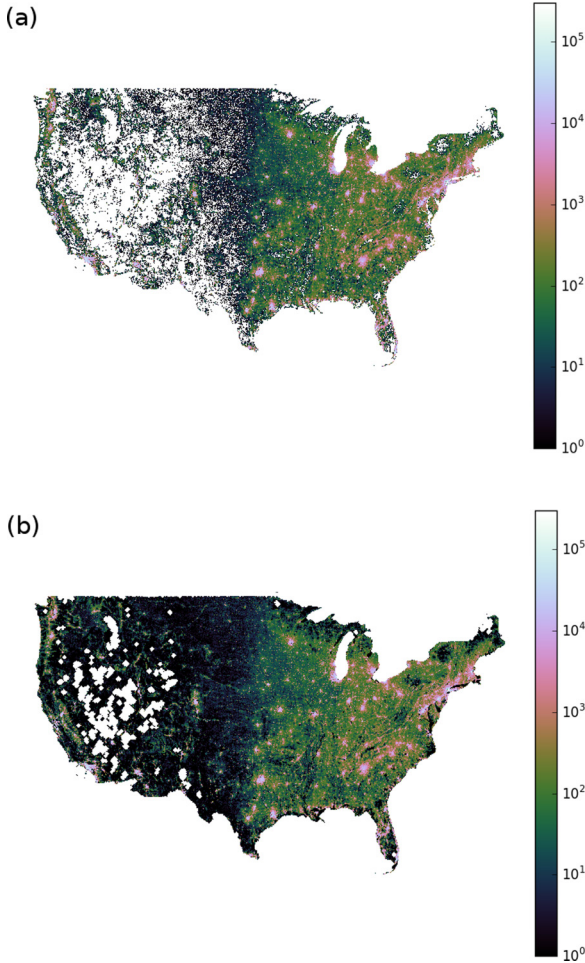
FIG. 9. (Color online) (a) 1500 \times 900 grid of the 2010 US Census Data showing raw data. Notice the multitude of squares with no people in them in the Western United States. (b) The resulting map after six steps of binary closing added to the original population.
