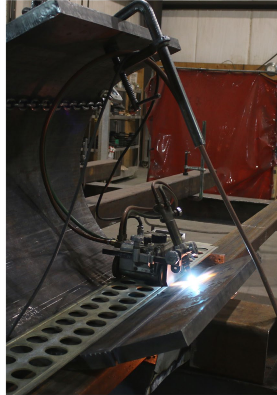
1.5" Plate Cylinder
