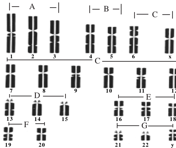
Fig. 4.1. Karyotyping of human chromosomes - pairs of chromosomes during metaphase
